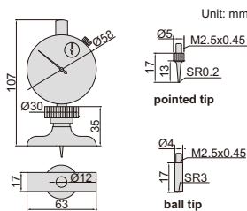
ball tip
