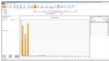
spectrum analysis
