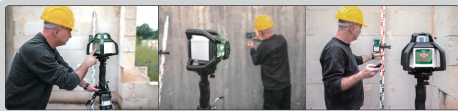
horizontal leveling
