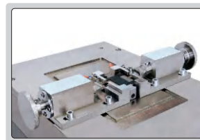
lowered broaches
