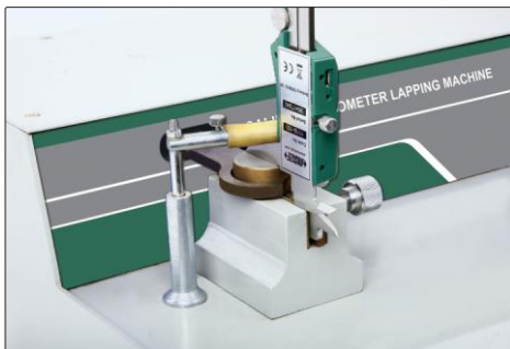
lapping measuring surfaces of caliper lower jaws
