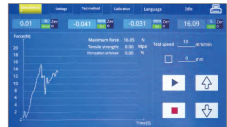
test interface
