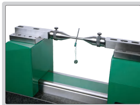
pin gauge measurement
